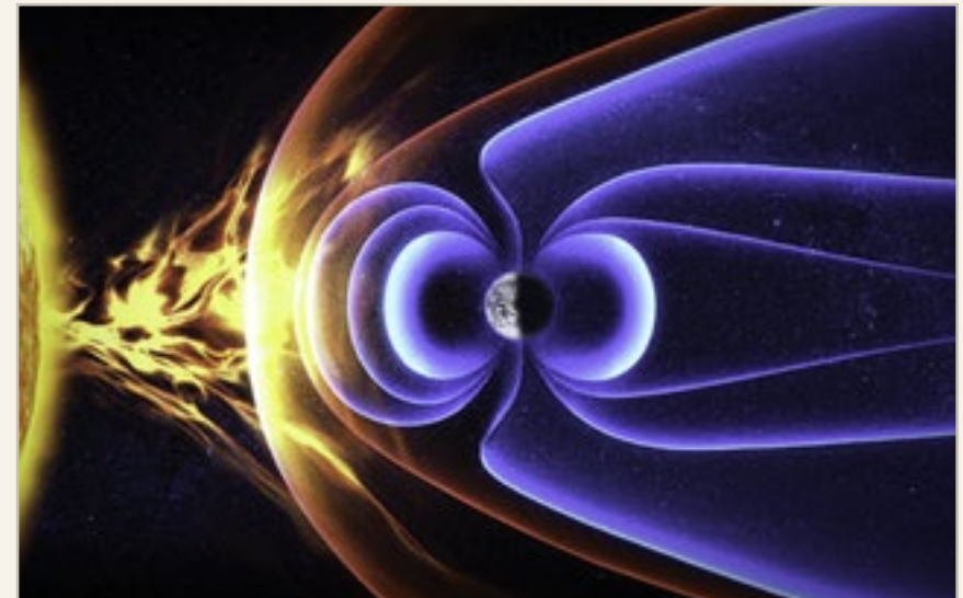
The Earth's expanding radiating equator and the contracting electric north and south poles.
